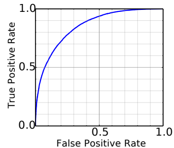
Figure 2: ROC curve for the Content + Context Model.
